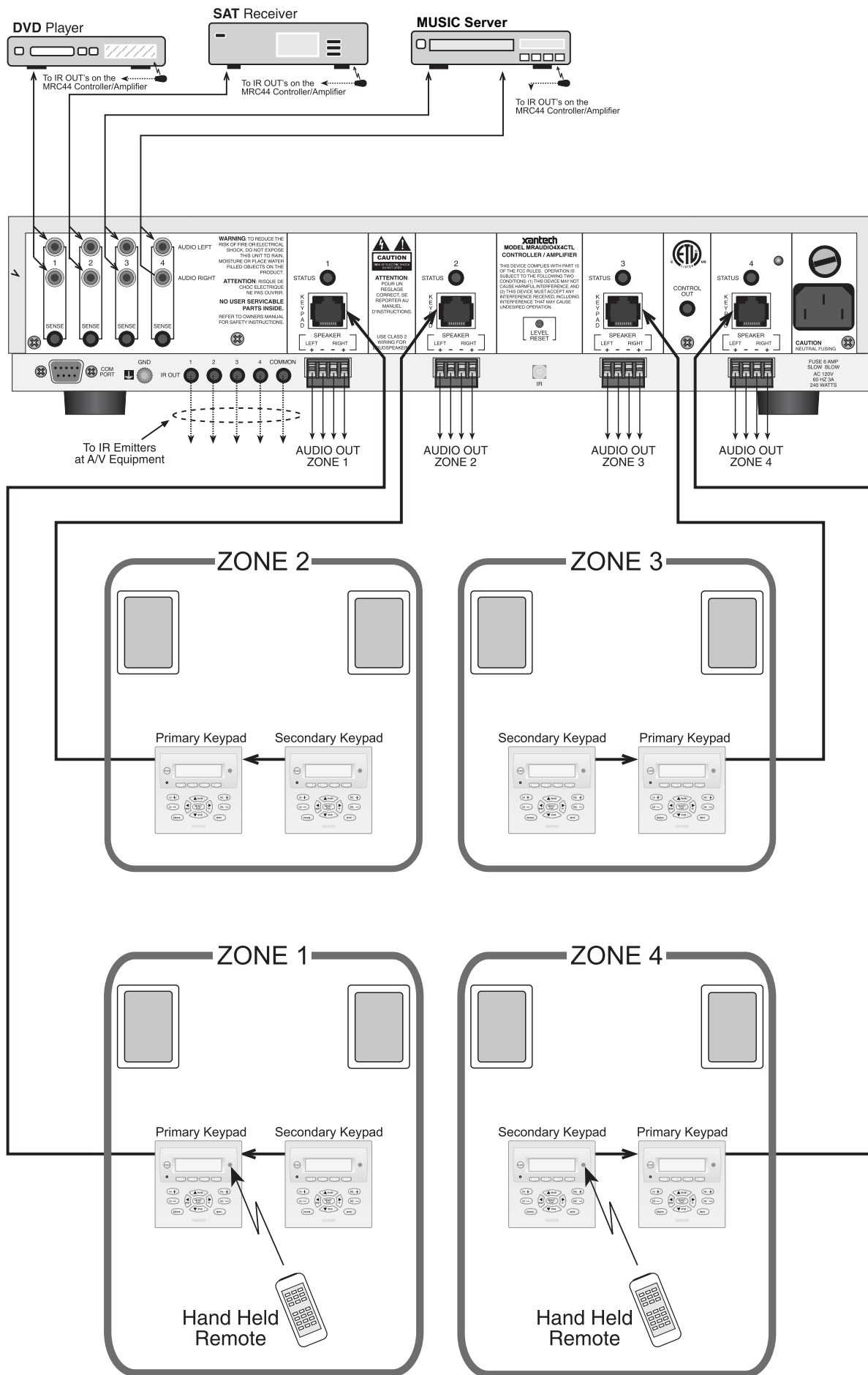
Figure 13 –Typical MRAUDIO4X4 System
